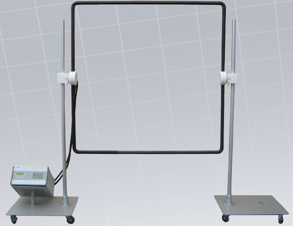
Magnetic Immunity Test System for IEC/EN61000-4-8
