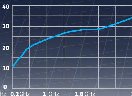
LP-02 - Antenna Factor
