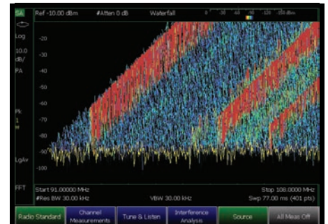
Waterfall display makes interference hunting easier
