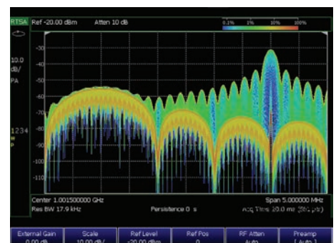
Multi-pulse detection with the density display
