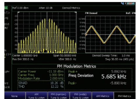
Characterize AM/FM signals using AM/FM demodulation
