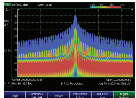
Density display with settable persistence
