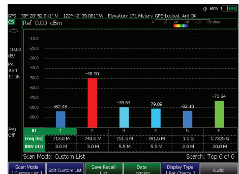
Scan up to 20 channel simultaneously with the channel scanner option
