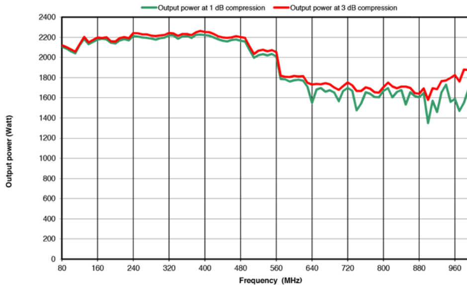
MT2000 POWER AMPLIFIER 2000W / 80 MHz - 1000 MHz
