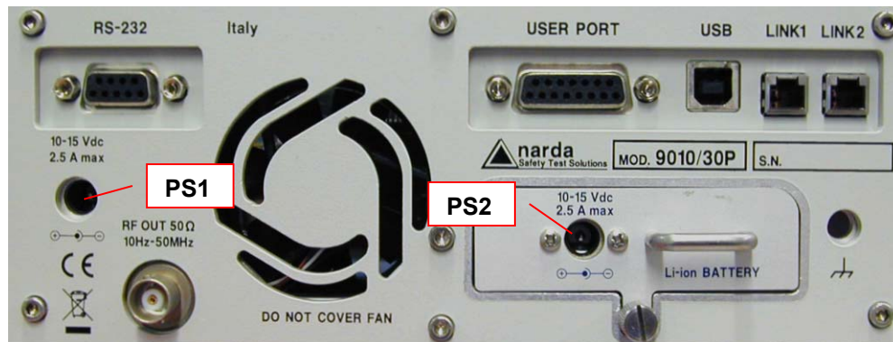
Fig. 9-5 Rear Panel
