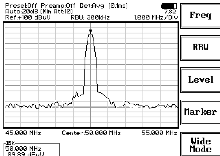
Fig. 11-17 Spectrum
