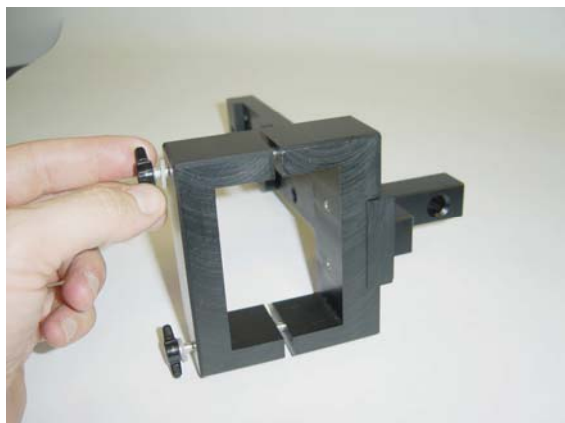
Fig. 11-9 Closing the Antenna Holder Periodic
