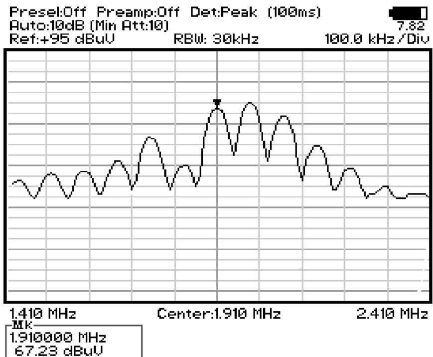
Fig. 5-1 Spectrum
