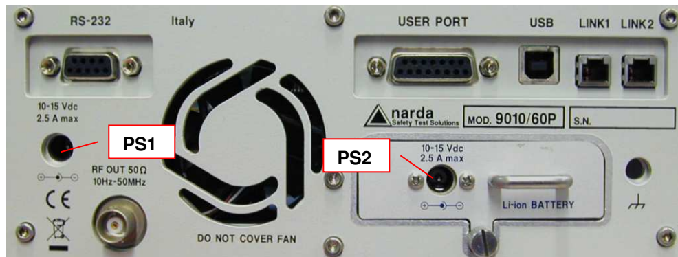
Fig. 9-8 Rear Panel
