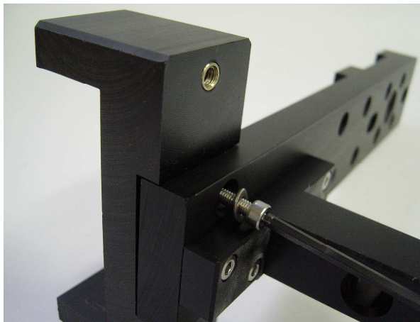
Closing the Antenna Holder and insert the Adapter for PMM Log-Periodic
