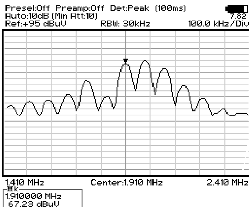
Fig. 5-1 Spectrum
