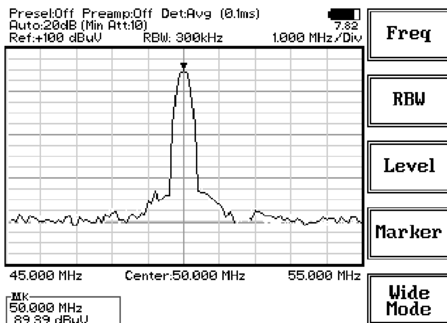
Fig. 11-8 Spectrum
