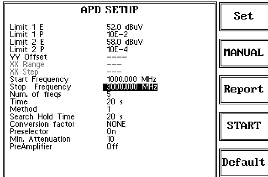
Fig. 4-1 APD Setup
