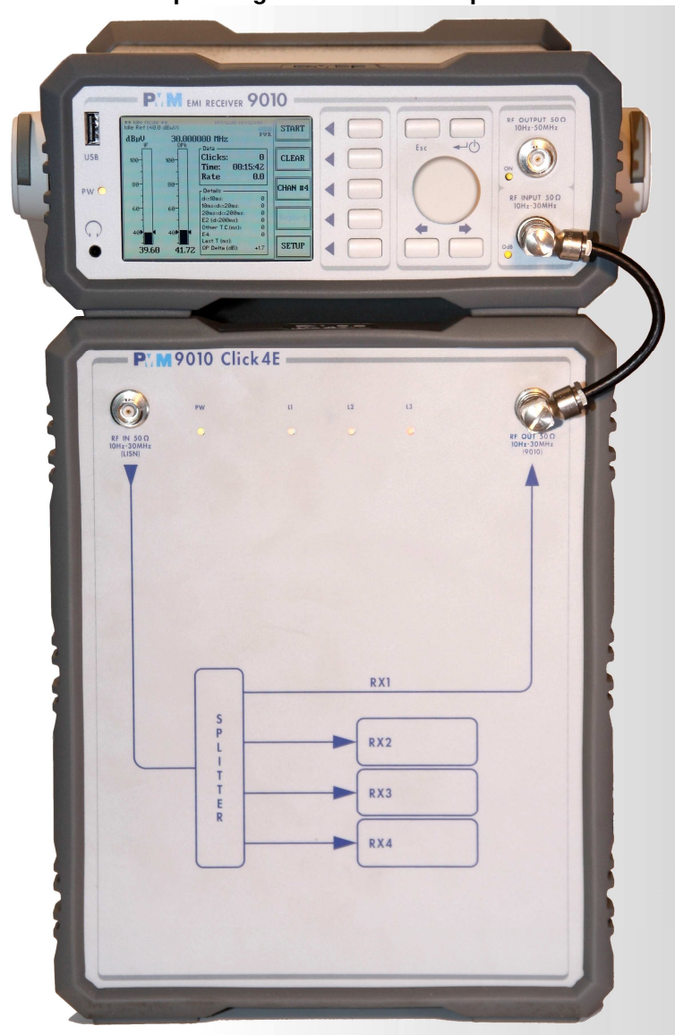
9010 and 9010 Click4E Option system front view
