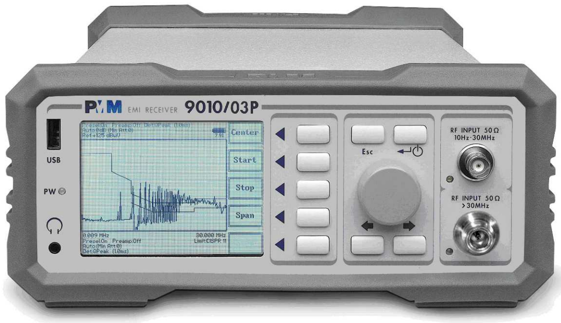
Fig. 9-1 Front Panel
