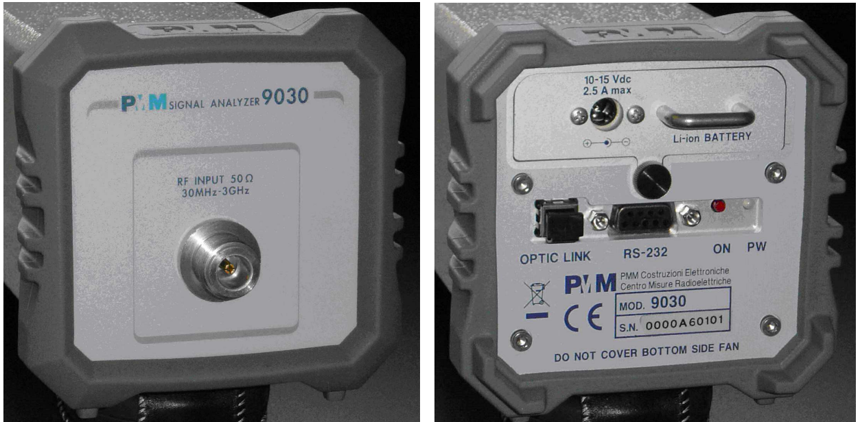
Fig. 11-1 9030 Front and Rear Panels
